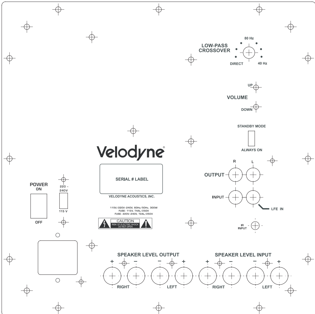
Figure 3. DEQ-15R Rear Panel Connections
